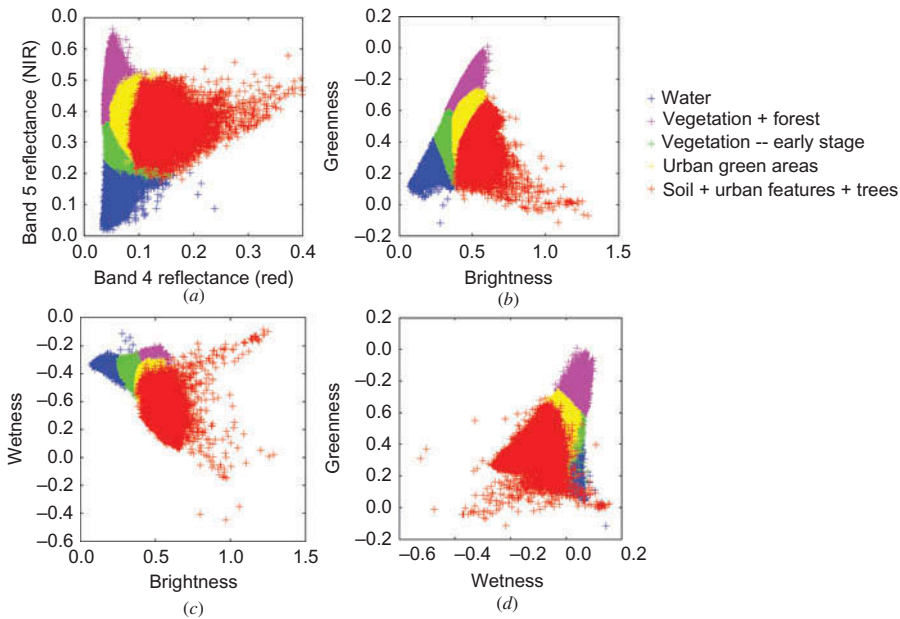
Figure 1. (a) Scatter plot between Red (band 4) and NIR bands (band 5) along with all five regions of interests (ROIs); (b) Scatter plot between Brightness and Greenness. It is also called ‘plane of vegetation’; (c) Scatter plot between Brightness and Wetness. It is also termed as ‘plane of soil’; (d) Scatter plot between Wetness and Greenness. It is called as ‘transition zone’.
